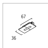
Straight coupler to join two sections of track electrically. For static reason order mechanical coupler (page 20/21) if suspended via pendant rod or wire
